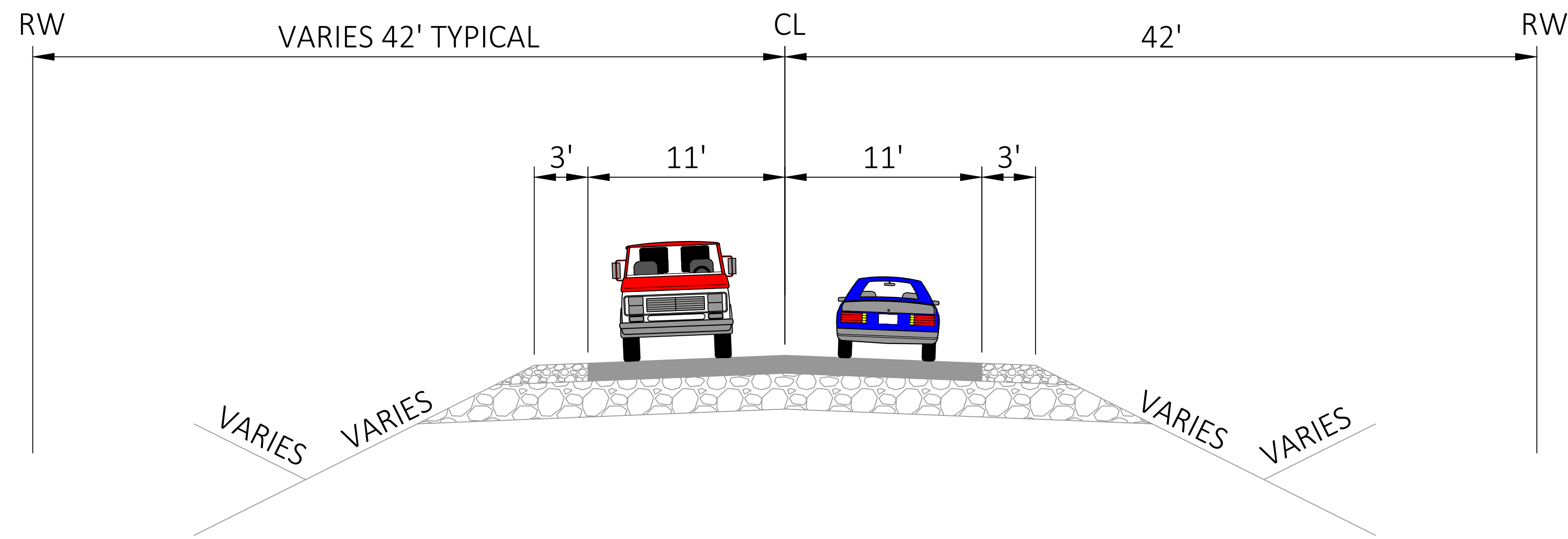
EXISTING TYPICAL SECTION COUNTY A
