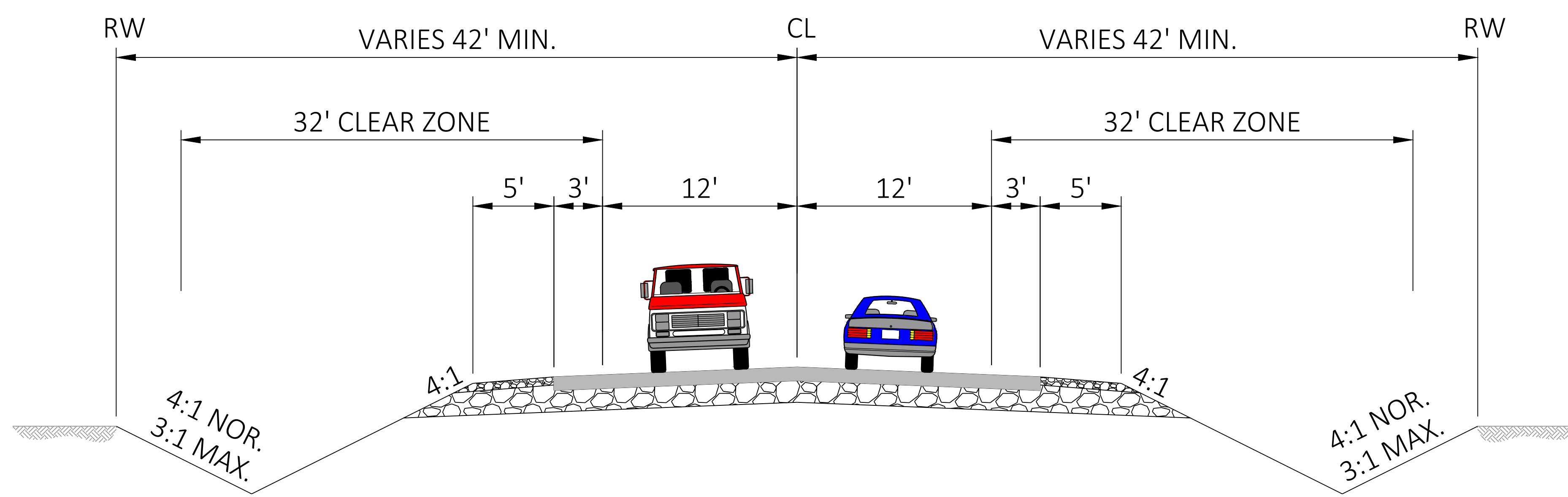
FINISHED TYPICAL SECTION COUNTY A
